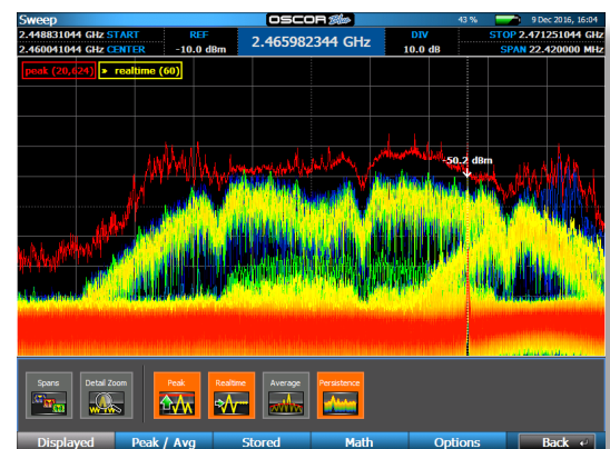
Persistence display
